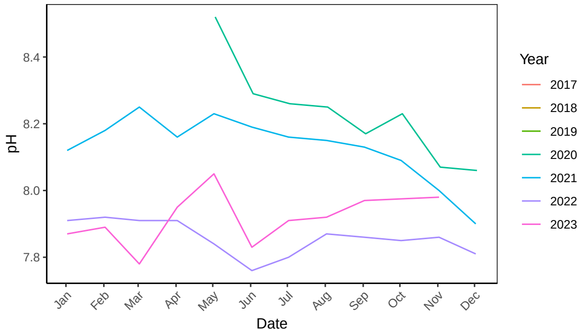
B2 Raceway 1 pH Monthly Statistics
